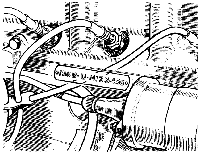
Engine Number (later models). This is stamped on a plate on the right-hand side of the cylinder block
